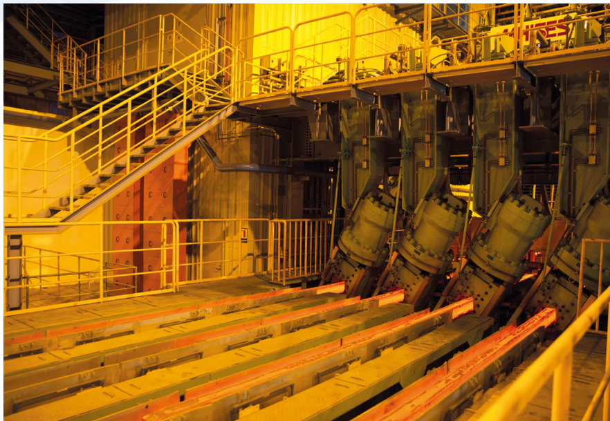
STEEL BILLETS
